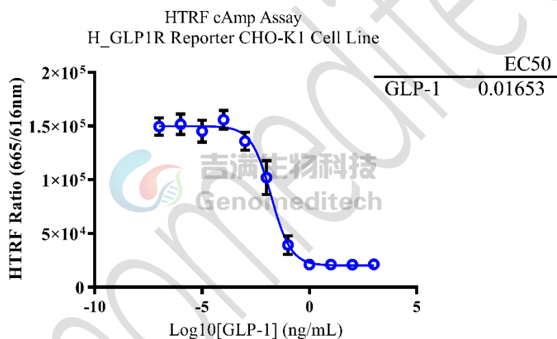
Figure 6 | H_GLP1R Reporter CHO-K1 cells were seeded at a density of 7500 cells per well in white 384-well microplates (5 \mu L per well). Gradient-diluted human GLP-1 solutions were then added, and the cells were incubated at room temperature for 30 minutes. The HTRF cAMP Gs Dynamic Detection Kit (Revvity, Cat. No. 62AM4PEB) was used according to the manufacturer's instructions. Fluorescence signals were measured using a Molecular Devices i3x multi-mode plate reader with excitation at 340 nm and emissions detected at 616 nm and 665 nm. The data were expressed as the 665 nm/616 nm \times 100,000 (HTRF Ratio) and used to calculate the EC50 value.
