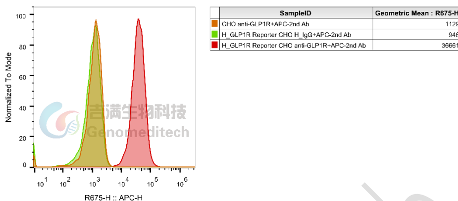
Figure 5 | H_GLP1R Reporter CHO-K1 Cell Line (Cat. GM-C09150) was determined by flow cytometry using Anti-GLP1R hIgG1 Antibody(mAb-36986)(Cat. GM-51168AB ).
