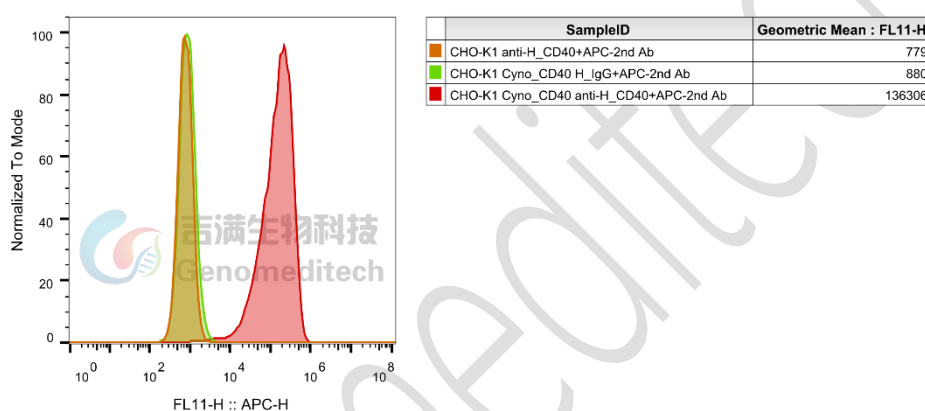
Figure 1 | Cynomolgus_CD40 CHO-K1 Cell Line (Cat. GM-C09602) was determined by flow cytometry using Anti-H_CD40 hIgG1 Antibody (Cat. GM-24025AB ).
