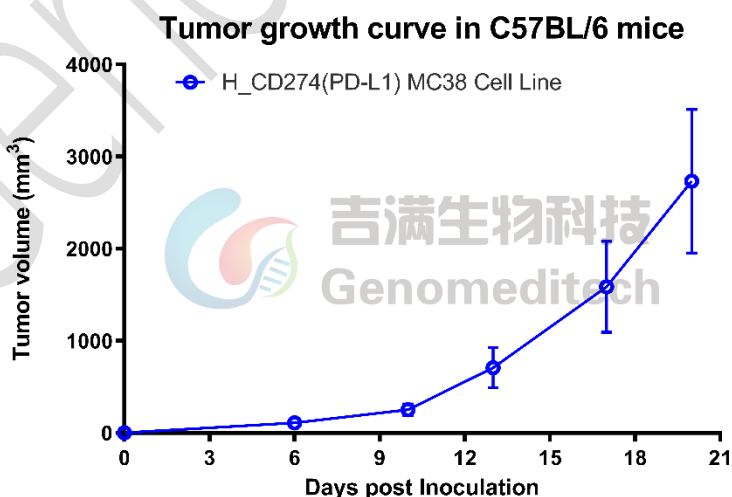
Figure 2 | Tumor growth curves of H_CD274(PD-L1) MC38 in C57BL/6 mice. H_CD274(PD-L1) MC38 cells ( 1 \times 10^6 per mouse) were subcutaneously inoculated into C57BL/6 mice (female, 8 weeks old, n = 3 ). Tumor volume was measured twice per week and is presented as mean \pm SEM.
