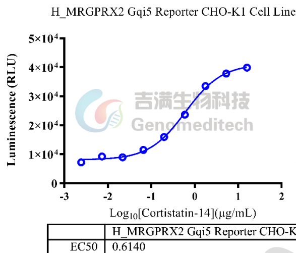
Figure 1 | Response to Cortistatin-14. The H_MRGPRX2 Gqi5 Reporter CHO-K1 Cell Line (Cat. GM-C37885) at a concentration of 1E4 cells/well (96-well format) was stimulated with serial dilutions of Cortistatin-14 (MCE/HY-P1932) in assay buffer (F12K+1% FBS+1% P.S) for 6 hours. The firefly luciferase activity was measured using the Luciferase Reporter Assay Kit (Genomeditech). The maximum induction fold was approximately [5.7]. Data are shown by drug mass concentration.
