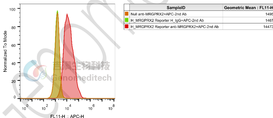
Figure 4 | H_MRGPRX2 Gqi5 Reporter CHO-K1 Cell Line (Cat. GM-C37885) was determined by flow cytometry using APC anti-human MRGX2 Antibody (Biolegend/359005).
