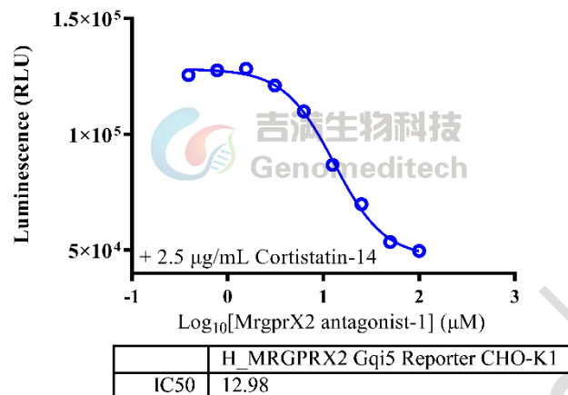
Figure 3 | Response to MrgprX2 antagonist-1. Serial dilutions of the MrgprX2 antagonist-1(MCE/HY-145191) was incubated with 1E4 cells/well of the H_MRGPRX2 Gqi5 Reporter CHO-K1 Cell Line (Cat. GM-C37885) in a 96-well plate for 1 hour in assay buffer (F12K+1% FBS+1% P.S). Subsequently, the Cortistatin-14 (MCE/HY-P1932) at a concentration of 0.25 μg/well was added, and the coculture proceeded for an additional 6 hours. Firefly luciferase activity was then measured using the Luciferase Reporter Assay Kit (Genomeditech). The results indicated maximum blocking folds of approximately [2.6]. Data are shown by drug molar concentration.
