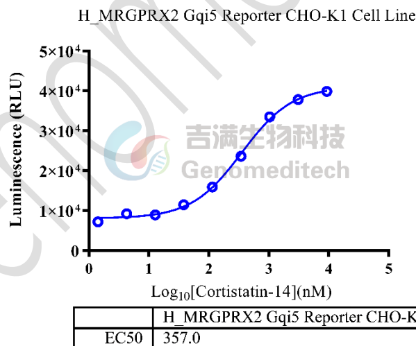
Figure 2 | Response to Cortistatin-14. The H_MRGPRX2 Gqi5 Reporter CHO-K1 Cell Line (Cat. GM-C37885) at a concentration of 1E4 cells/well (96-well format) was stimulated with serial dilutions of Cortistatin-14 (MCE/HY-P1932) in assay buffer (F12K+1% FBS+1% P.S) for 6 hours. The firefly luciferase activity was measured using the Luciferase Reporter Assay Kit (Genomeditech). The maximum induction fold was approximately [5.7]. Data are shown by drug molar concentration.
