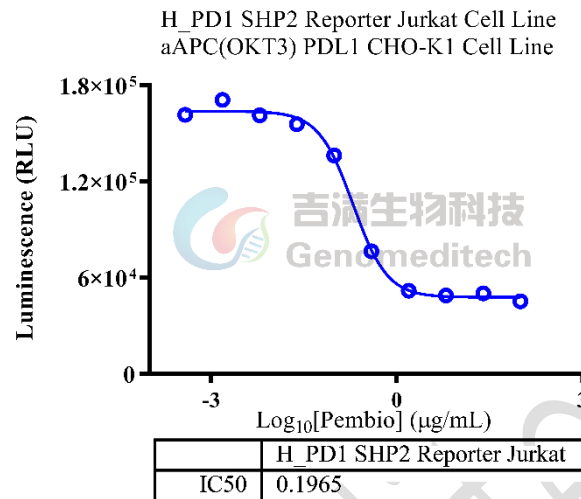
Figure 3 | Response to Anti-PD1 hIgG4 Reference Antibody (Pembio). aAPC(OKT3) PDL1 CHO-K1 Cell Line (Cat. GM-C05269 ) was seeded at a density of 1.5E4 cells/well in a 96-well plate and incubated overnight. The next day, serial dilutions of the Anti-PD1 hIgG4 Reference Antibody (Pembio) (Cat. GM-87802MAB ) were incubated with 1E5 cells/well of the H_PD1 SHP2 Reporter Jurkat Cell Line (Cat. GM-C42136 ) in a 96-well plate for 1 hour, and then added to the pre-seeded cells. The mixture was incubated for an additional 6 hours. Luciferase activity was measured using the Luciferase Assay System. The results indicated a maximum fold of approximately [3.1]. Data are shown by drug mass concentration.
